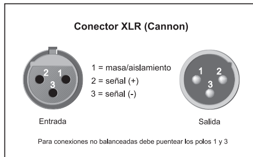
Fig. 5.2: Conector XLR
