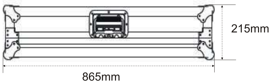
Front view
